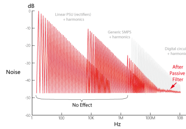
Equipment Generated Noise Reduction Passive Filter
