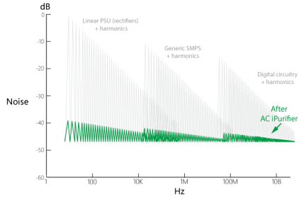
Equipment Generated Noise Reduction iFi AC iPurifier
